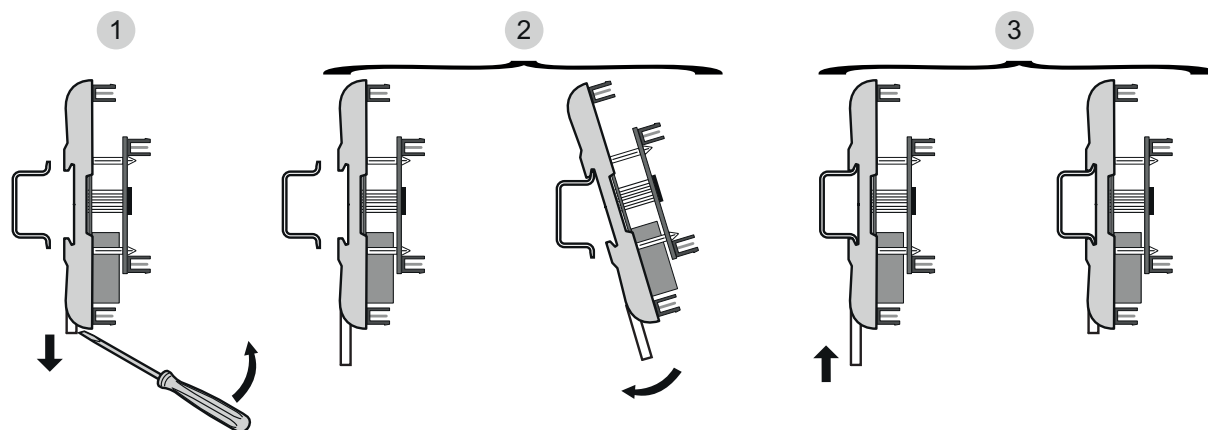
NSYSR200 IEC/EN60715
